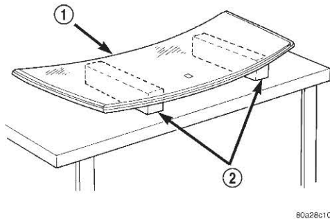
Fig. 3 Work Surface Set up and Molding Installation
