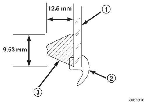
Fig. 4 Urethane Bead
